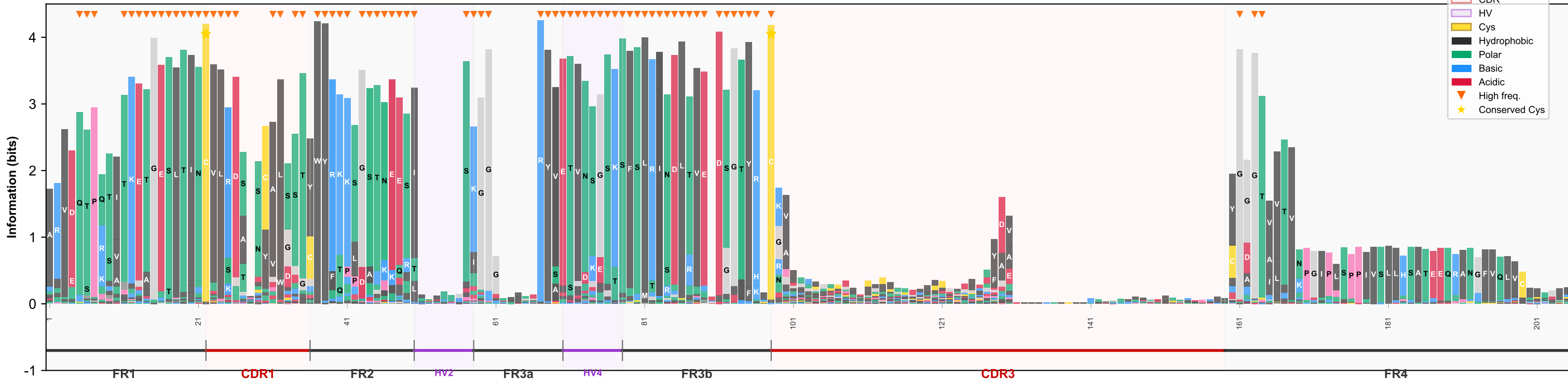
VNAR Sequence Logo — 260-Sequence MSA (205 columns) FR1-CDR1-FR2-HV2-FR3a-HV4-FR3b-CDR3-FR4
