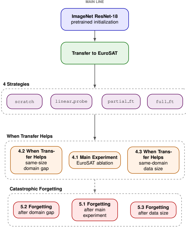
Figure 1. Experimental workflow used in Sections 4 and 5. The downstream experiments compare transfer strategies, target-domain distance, and training-set size. The downstream-trained checkpoints are then re-evaluated on ImageNet to measure catastrophic forgetting.
