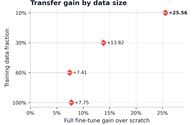
Figure 4. Same-domain data-size comparison. Left: EuroSAT test top-1 accuracy by training fraction. Right: transfer gain over training from scratch.
