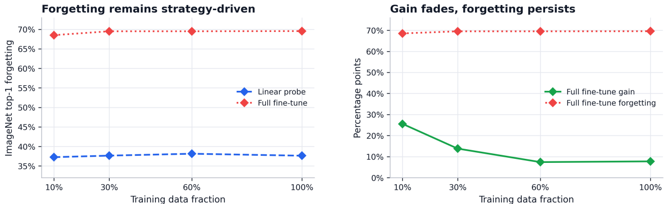
Figure 7. Forgetting after the data-size experiment. Left: ImageNet top-1 forgetting by transfer method. Right: transfer gain and forgetting trade-off.
