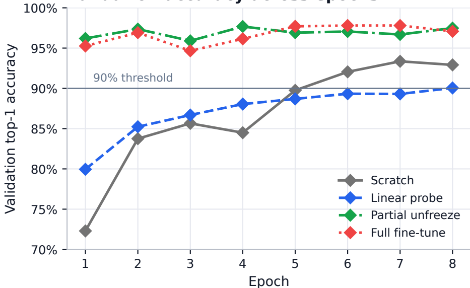
Validation accuracy across epochs
