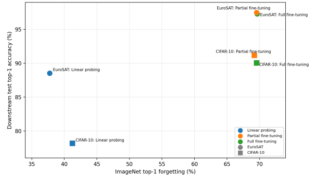
Figure 6. Forgetting after same-size downstream adaptation. Left: ImageNet top-1 forgetting. Right: downstream accuracy and ImageNet forgetting trade-off.
