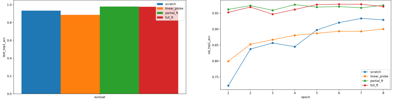
Figure 2. Side-by-side summary of Experiment 4.1. Left: final EuroSAT test top-1 accuracy by strategy. Right: validation top-1 trajectories across training epochs.
