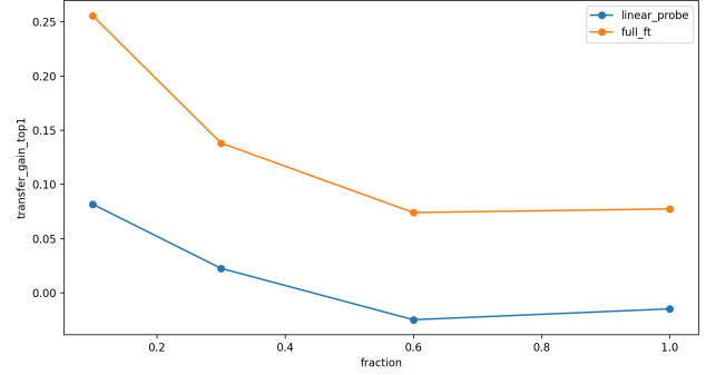
Figure 4. Same-domain data-size comparison. Left: EuroSAT test top-1 accuracy by training fraction. Right: transfer gain over training from scratch.
