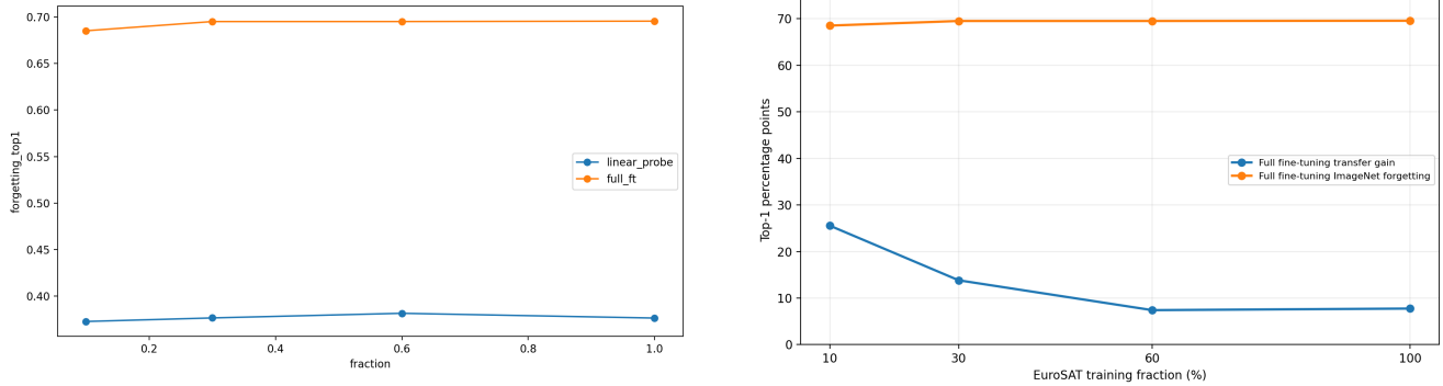
Figure 7. Forgetting after the data-size experiment. Left: ImageNet top-1 forgetting by transfer method. Right: transfer gain and forgetting trade-off.
