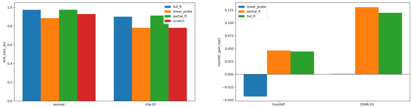
Figure 3. Same-size cross-domain comparison. Left: downstream test top-1 accuracy. Right: top-1 transfer gain over training from scratch.
