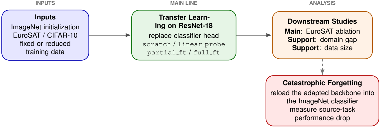
Figure 1. Experimental workflow used in Sections 4 and 5. The downstream experiments compare transfer strategies, target-domain distance, and training-set size. The downstream-trained checkpoints are then re-evaluated on ImageNet to measure catastrophic forgetting.
