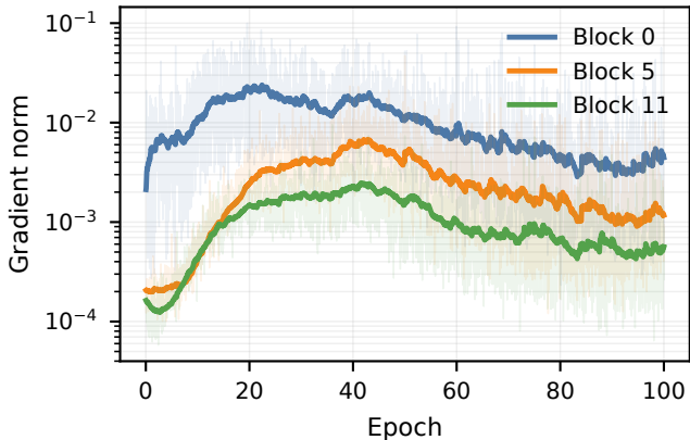
attn_quantizer.log_base_alpha
