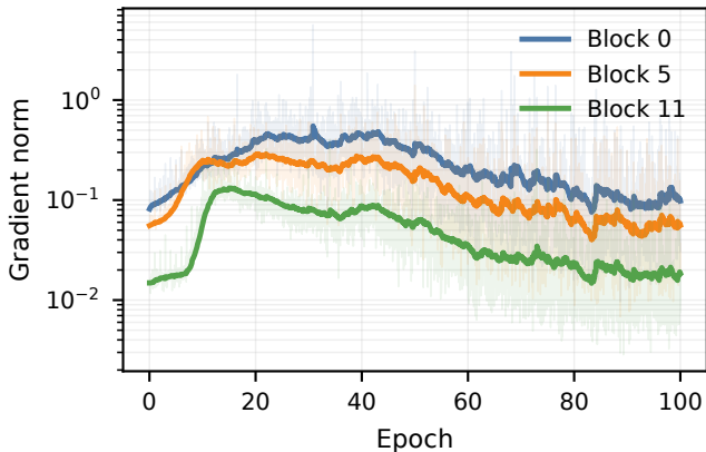
mlp.fc2.lora_B
