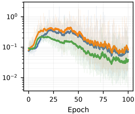
QKV LoRA-B gradient
