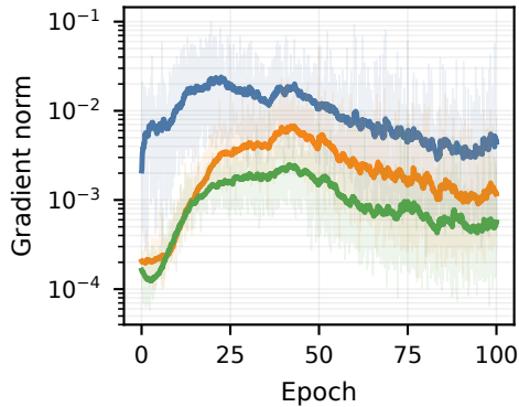
Attention log-base gradient
