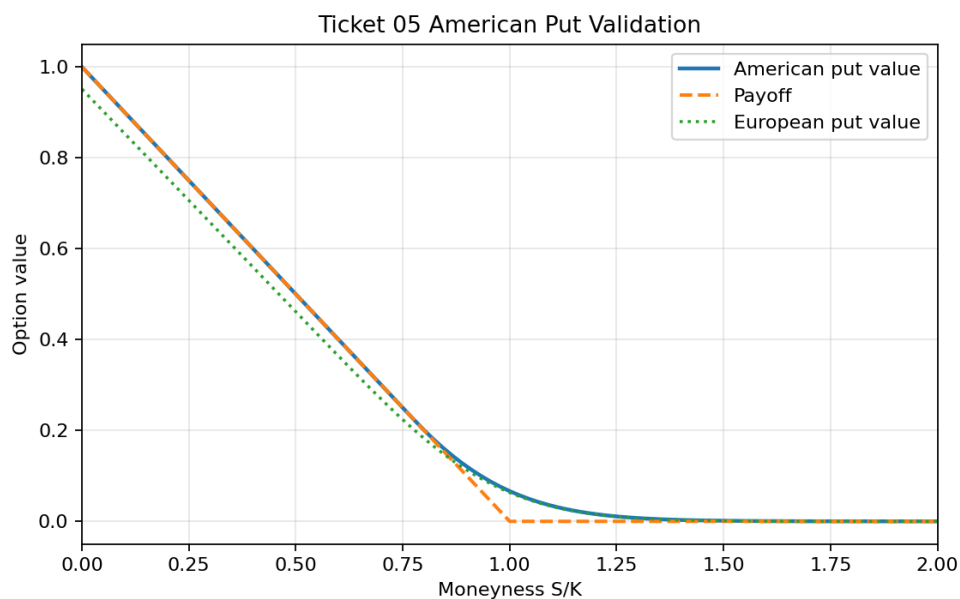
Figure 1: Ticket 05 American put value, payoff, and European put comparison. The plot is a validation visual, not a boundary-extraction plot.
