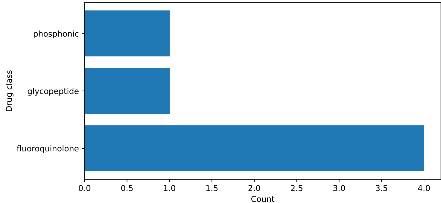
Barcode03: AMR hits by drug class
