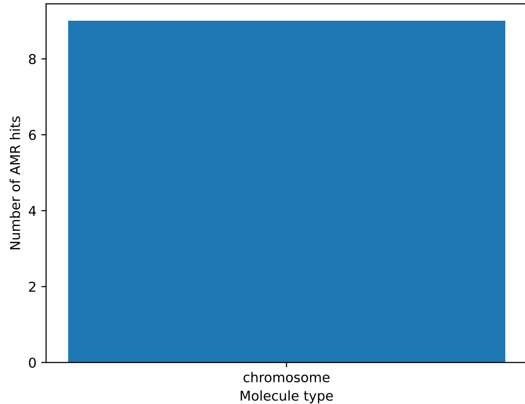
Barcode03: AMR hits by molecule type
