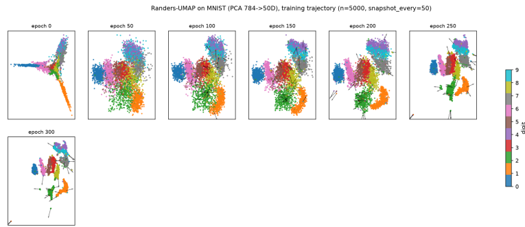
Figure 23: Snapshots of MNIST Embedding on 50-dim with 300 Epochs
