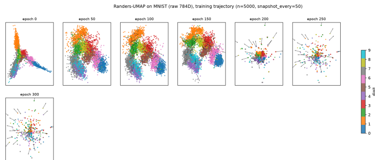
Figure 25: Snapshots of MNIST Embedding on 28x28-dim with 300 Epochs with gravity of strength 5
