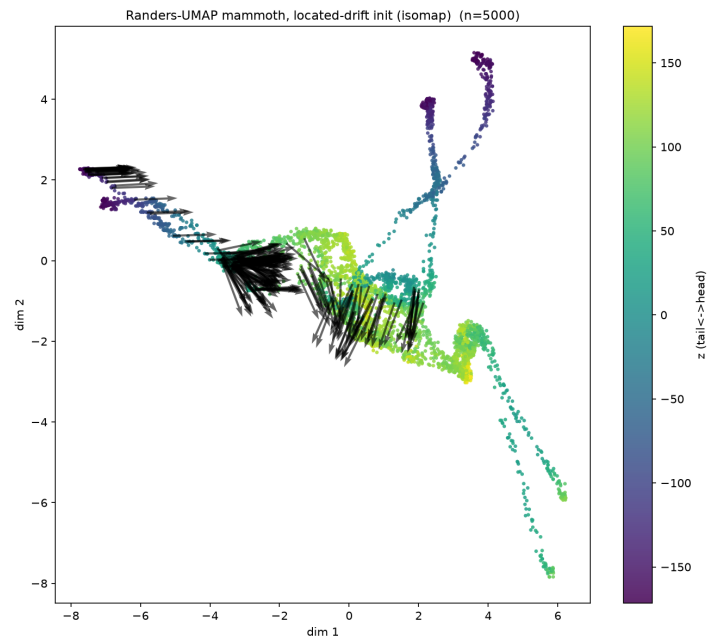
Figure 36: Mammoth Embedding with 50 epochs
