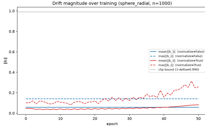
Figure 17: Drift Magnitude Graph for Sphere with Radial Drifts Embedding
