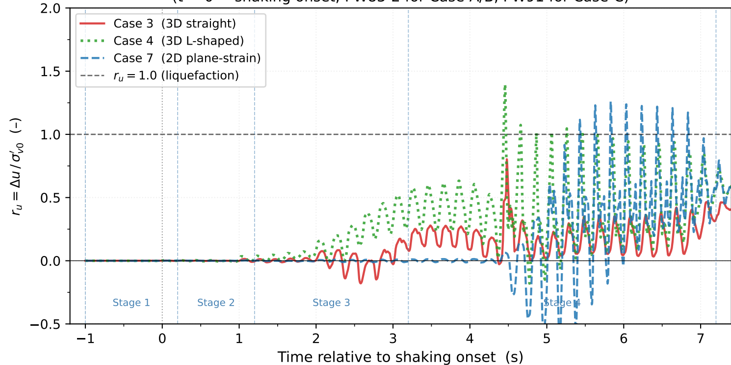
Beneath embankment crest r_u time histories — 25 mm depth ( t = 0 = shaking onset; PW83-2 for Case-A/B, PW91 for Case-C)
