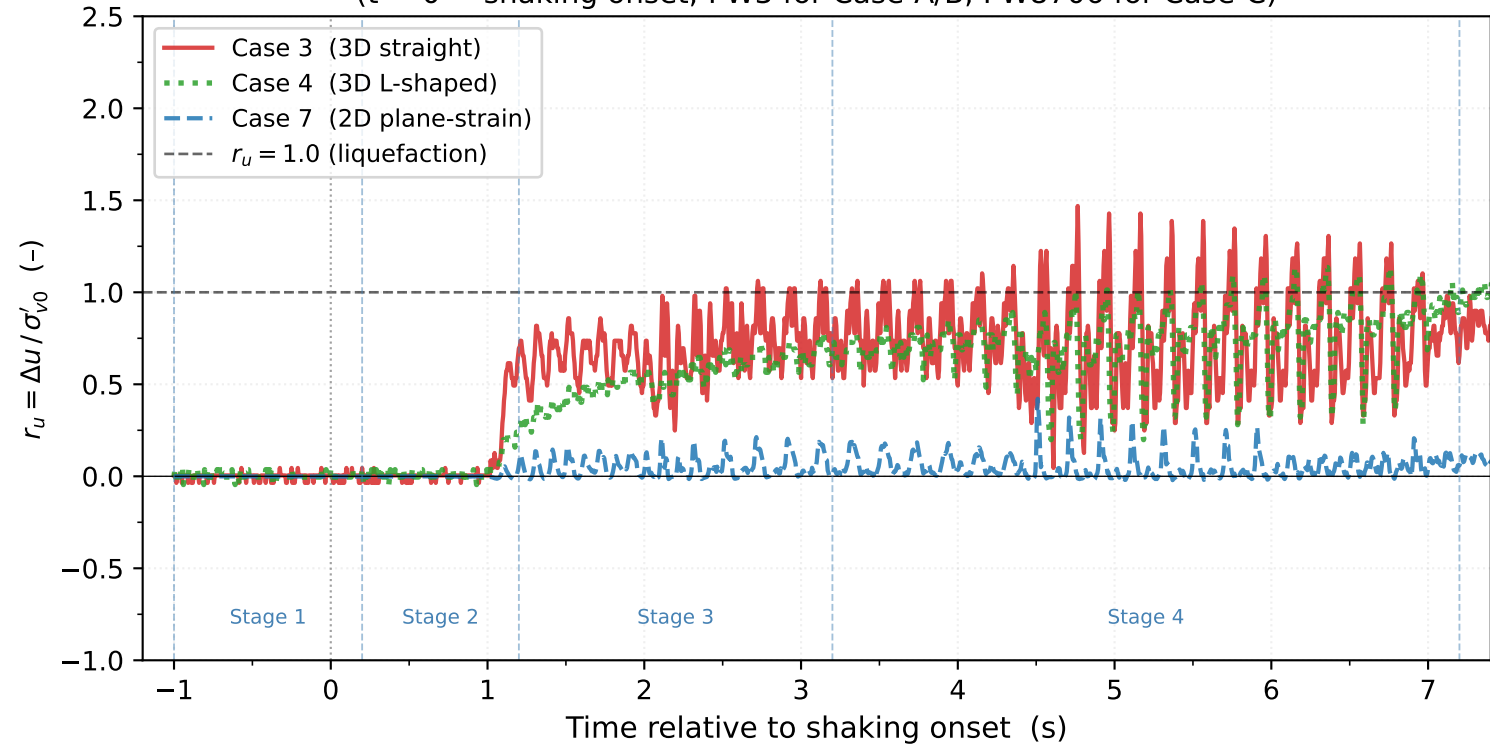
Free-field r_u time histories — 25 mm depth ( t = 0 = shaking onset; PW3 for Case-A/B, PW8706 for Case-C)
