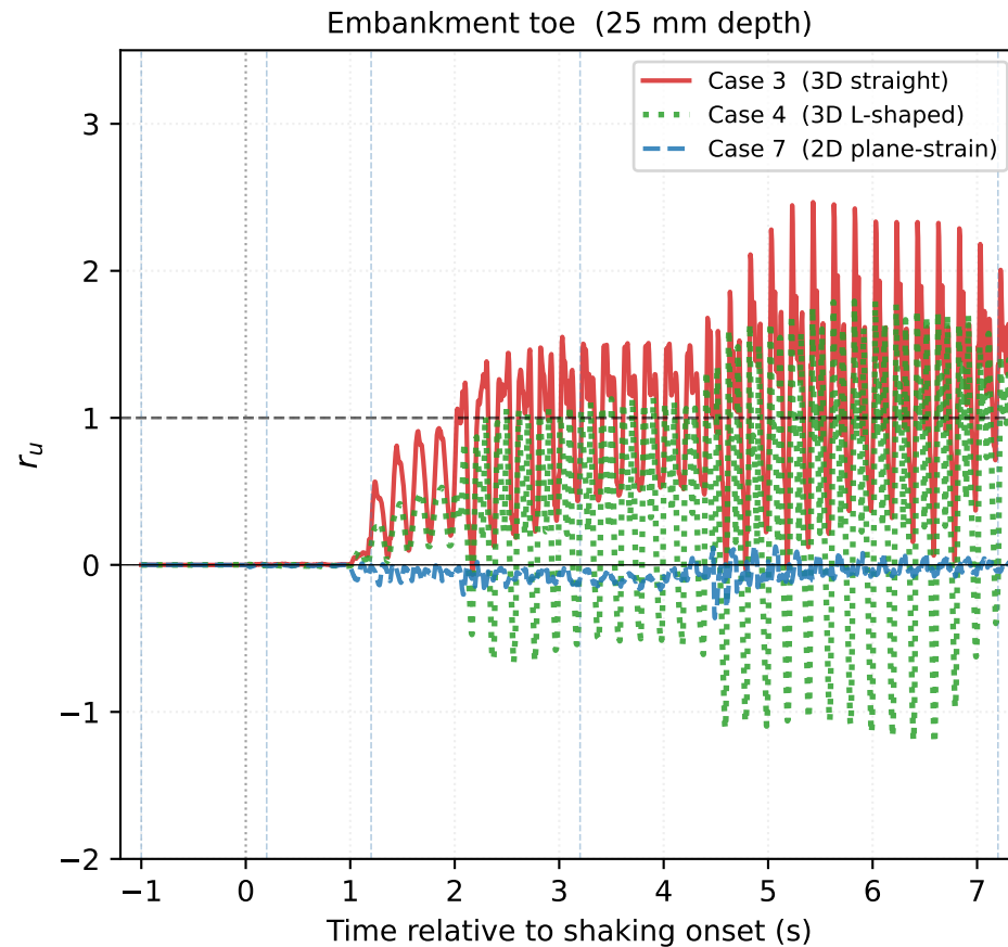
Time-aligned excess pore water pressure ratio r_u ( t = 0 = shaking onset) Free-field (25 mm) | Embankment toe (25 mm) | Beneath embankment crest (25 mm)
