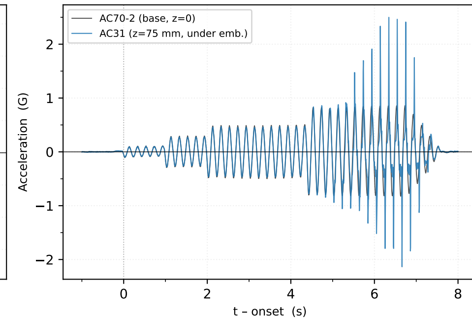
Acceleration comparison (base = black; soil at 75 mm = coloured)
