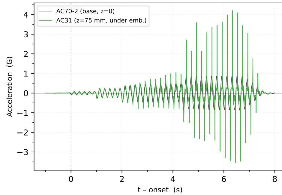
Acceleration comparison (base = black; soil at 75 mm = coloured)
