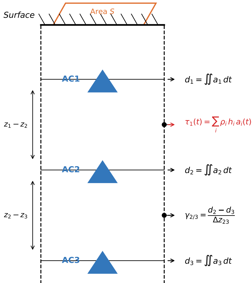
Figure 5 (revised): Procedure for shear strain and shear stress calculation from accelerometer data (Koga 1990; Watanabe 2023)
