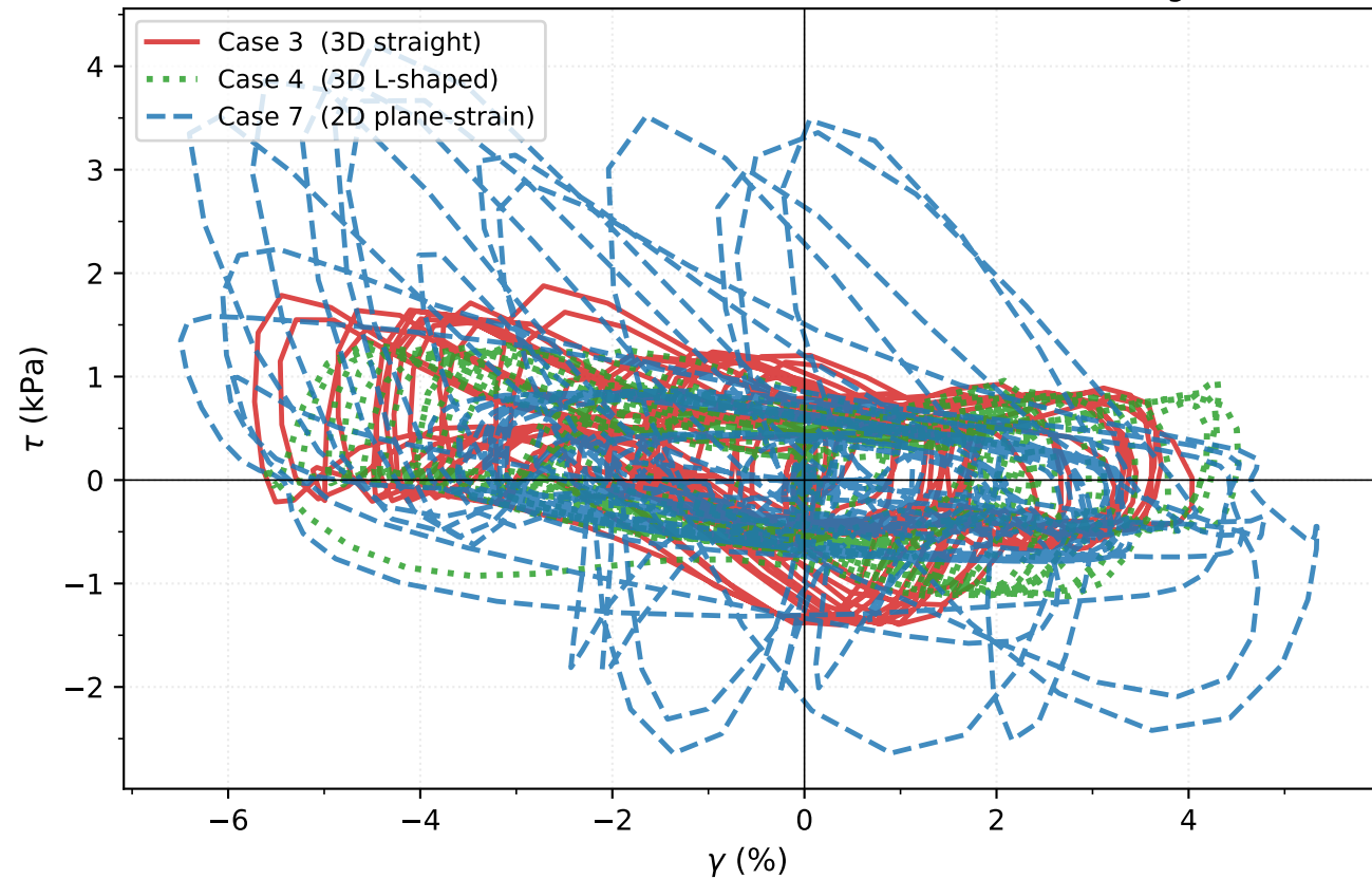
Shear Stress-Strain Loops — At Embankment Toe (AC24 \leftrightarrow AC25, \Delta z = 100 mm, no embankment surcharge)
