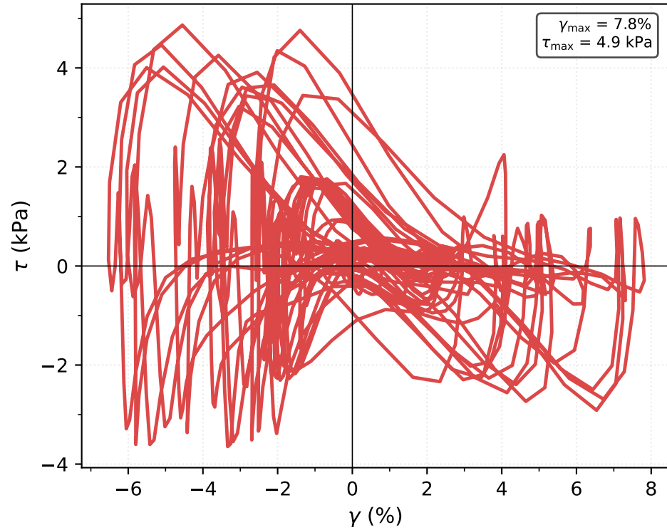
Case 3 (3D straight) At embankment toe
