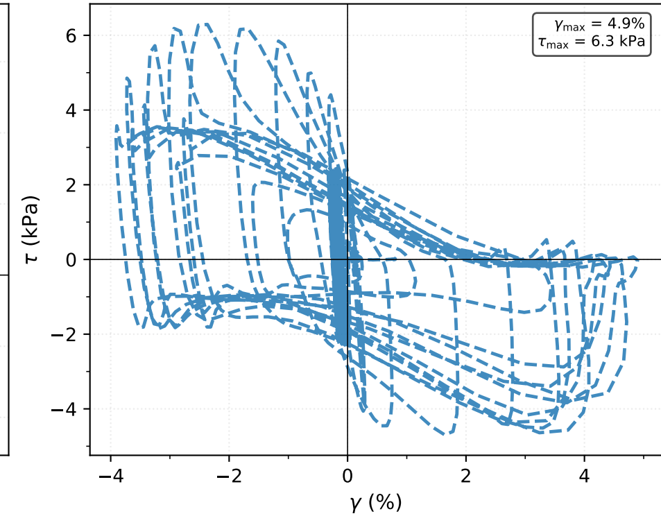
Case 7 (2D plane-strain) At embankment toe
