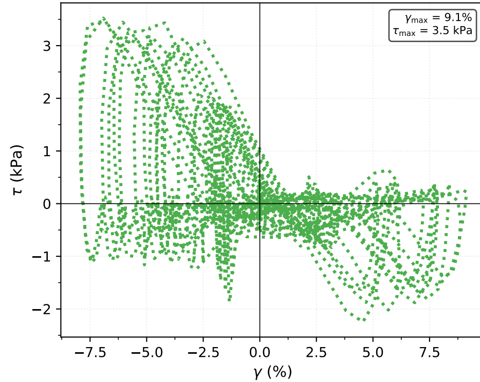
Case 4 (3D L-shaped) At embankment toe
