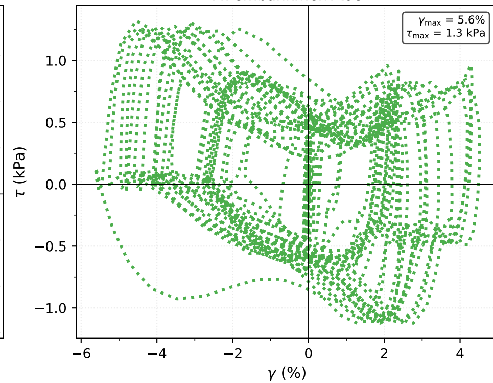
Case 4 (3D L-shaped) At embankment toe
