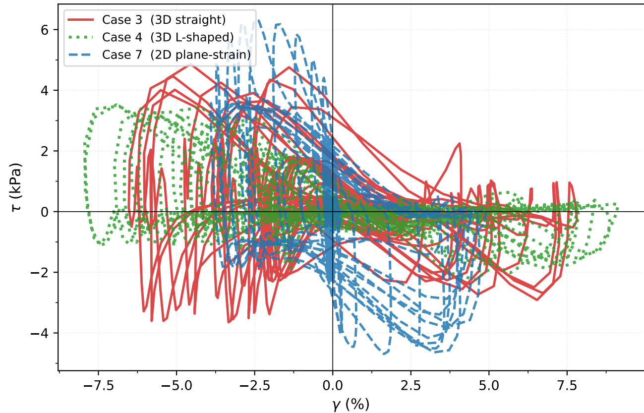
Shear Stress-Strain Loops — Beneath Embankment Crest (AC31 \leftrightarrow AC72-2/AC82, \Delta z = 100 mm)
