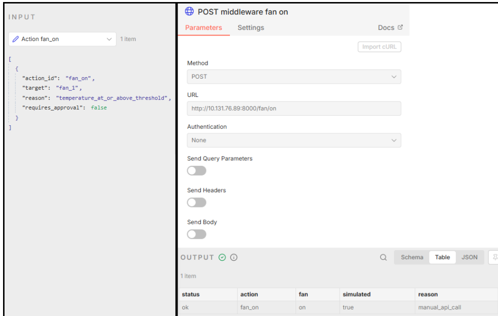
Figure 8: Raspberry Pi middleware/action-endpoint validation output for the high-temperature fan-on case.
