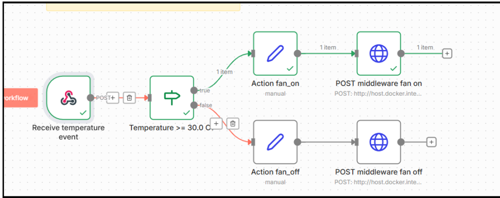
Figure 5: Deterministic baseline n8n workflow canvas.
