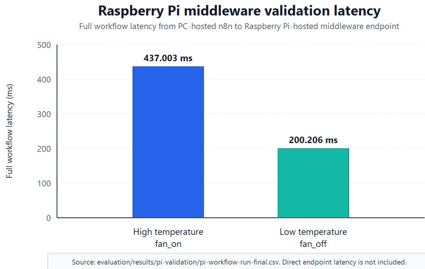
Figure 7: Raspberry Pi middleware/action-endpoint validation latency.
