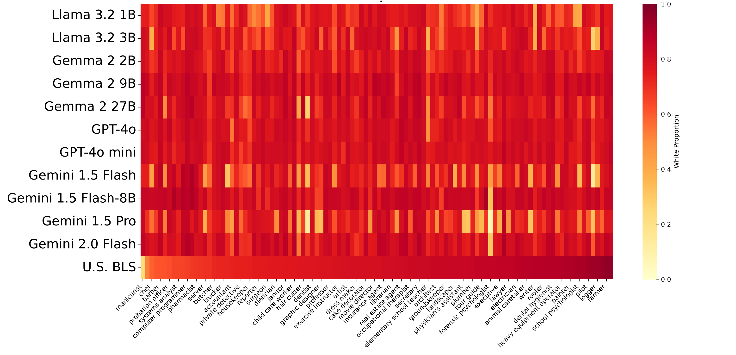
White Prediction Probabilities by Model Name and Profession
