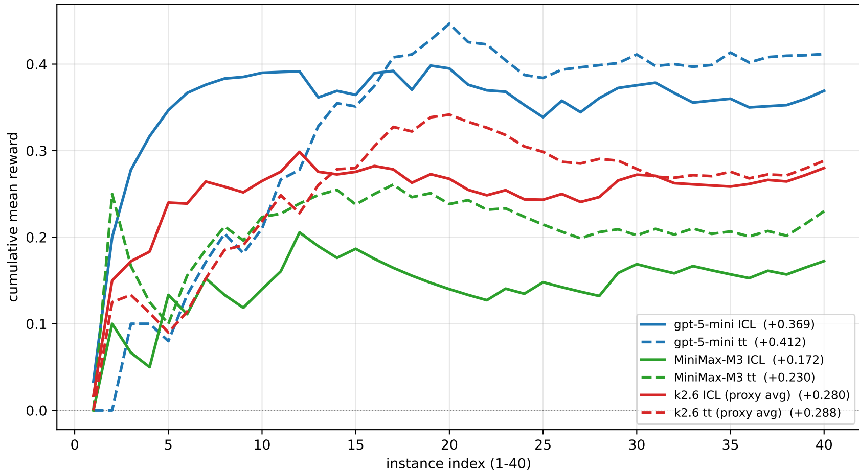
db - cumulative mean reward (2-seed avg)
