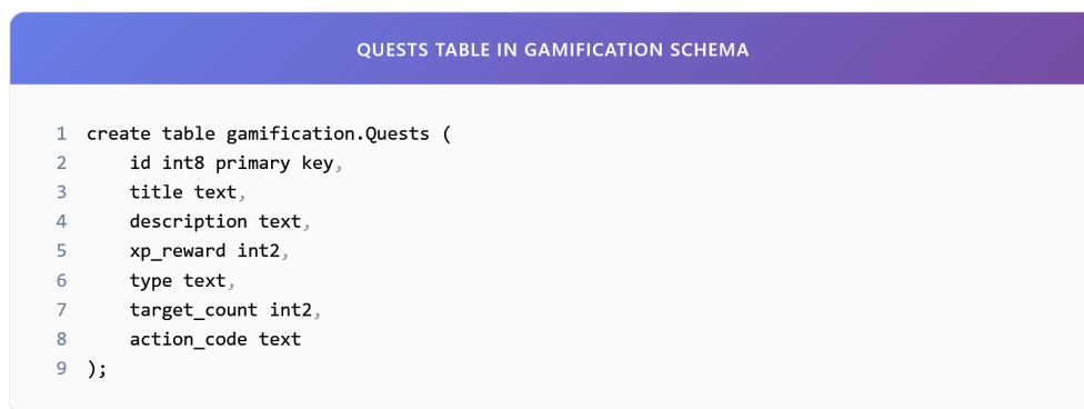
Abbildung 5.9: Quests table in gamification schema
