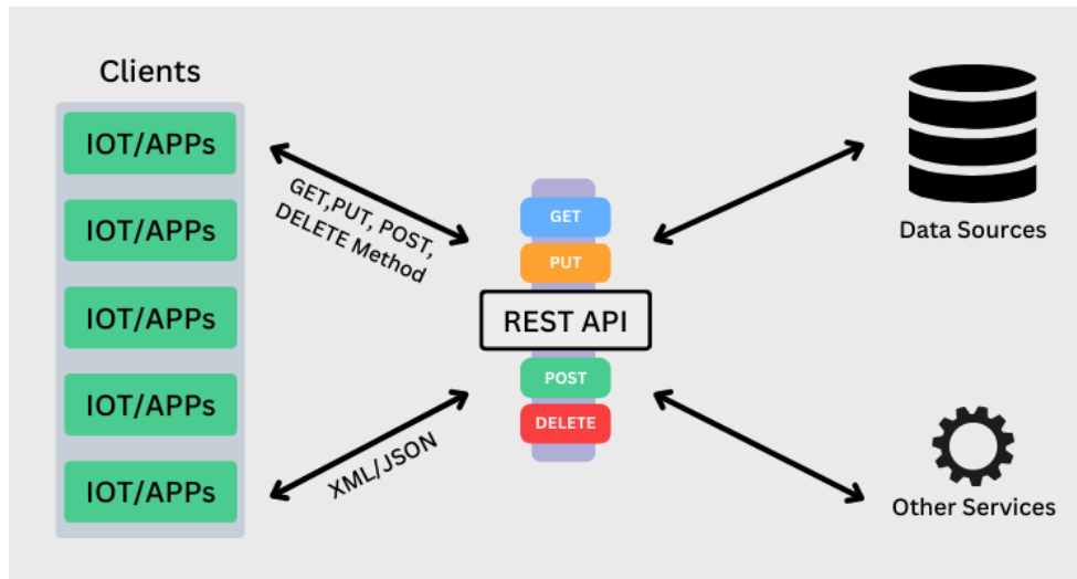
Abbildung 5.4: REST Request-Response Workflow: Stateless clients must open a new connection for every request, incurring significant overhead [31].
