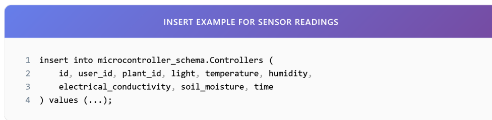
Abbildung 5.8: Insert operation for real-time sensor synchronization
