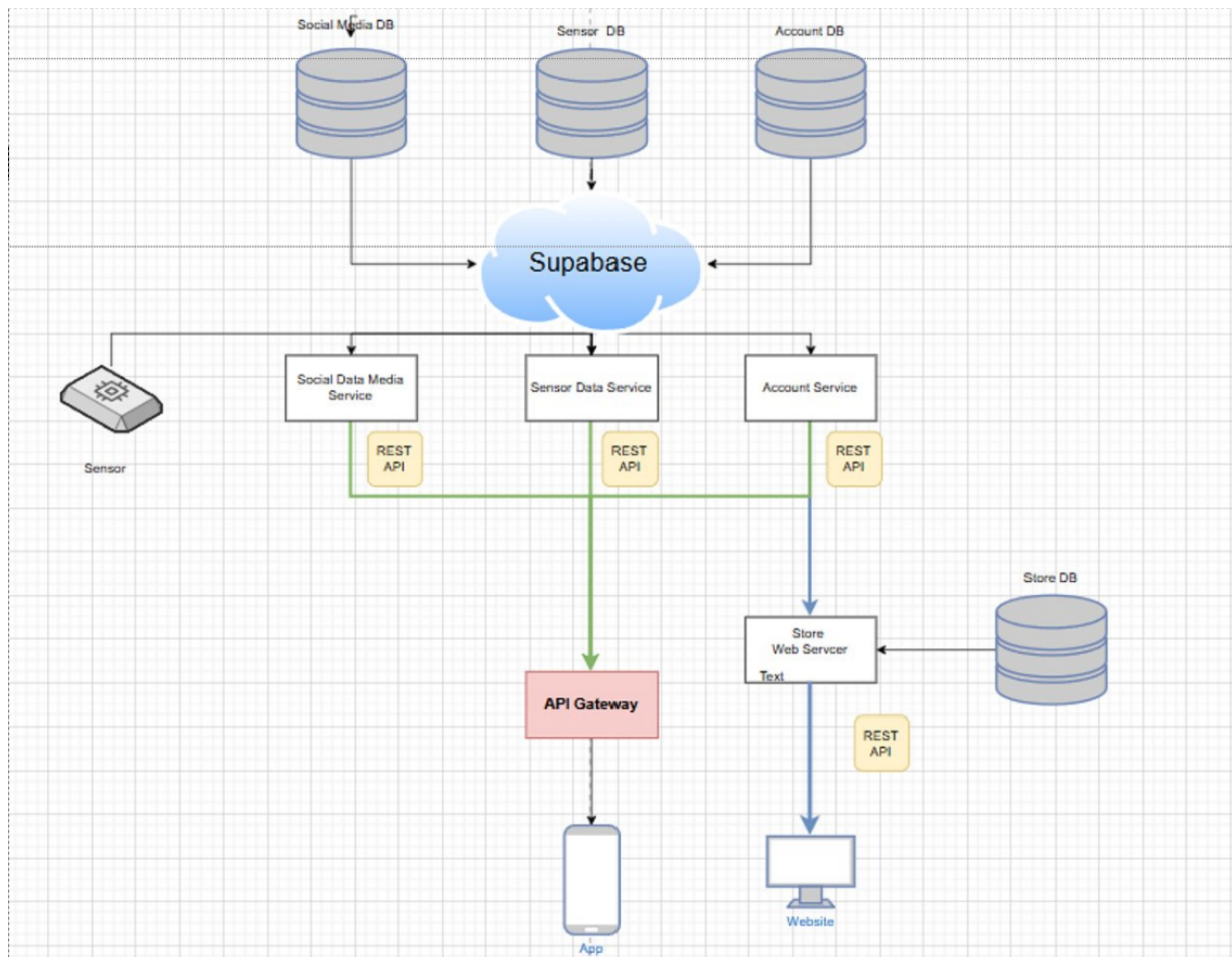
Abbildung 3.4: High-Level System Architecture Diagram (Source: Self-made)
