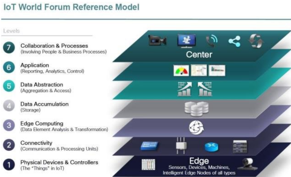
Abbildung 3.1: The 7-Layer IoT World Forum Reference Model [206]
