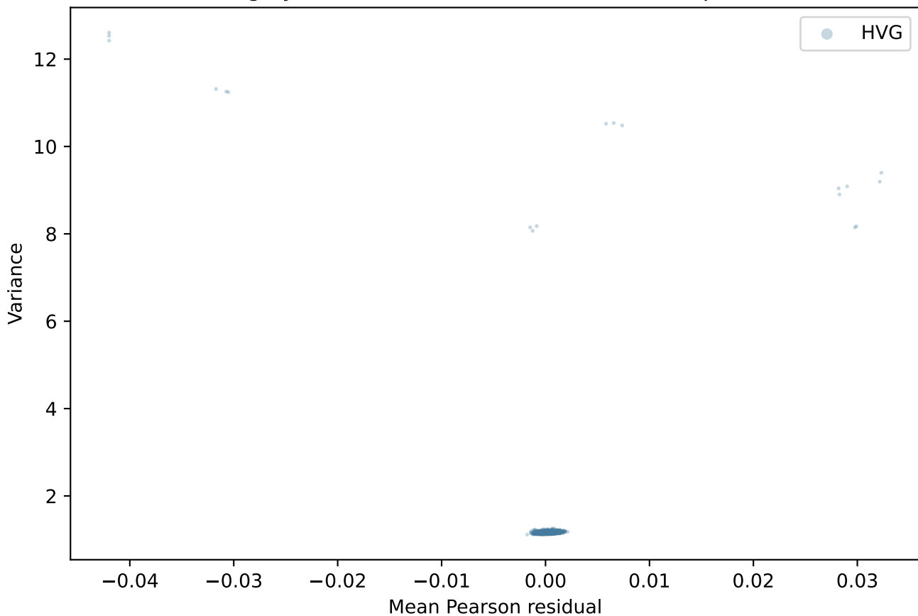
Highly Variable Genes (Pearson Residual space)
