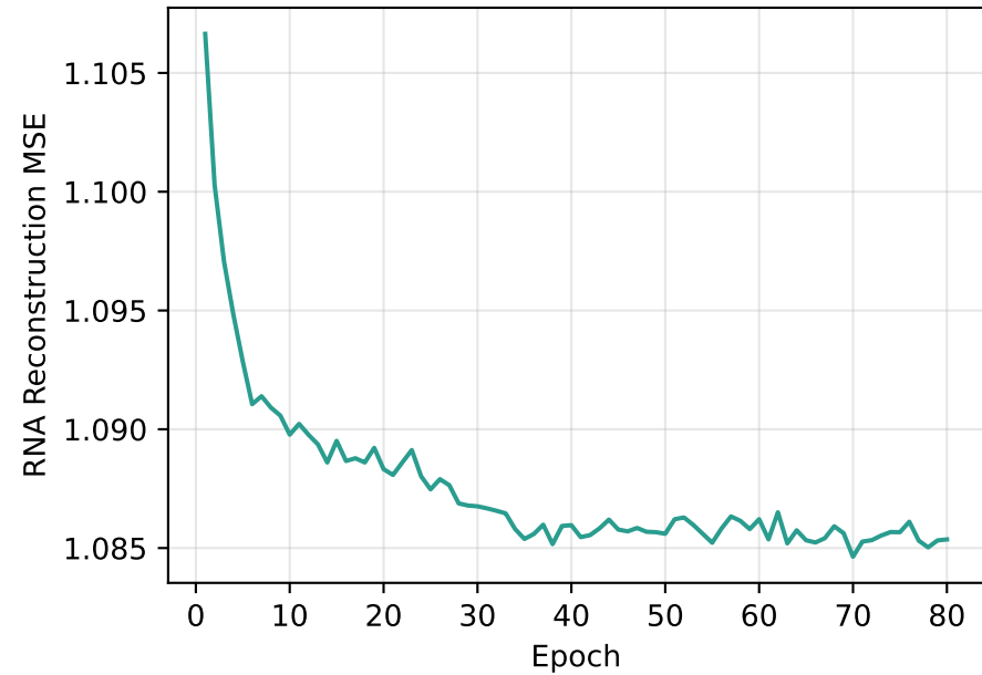
RNA Reconstruction MSE
