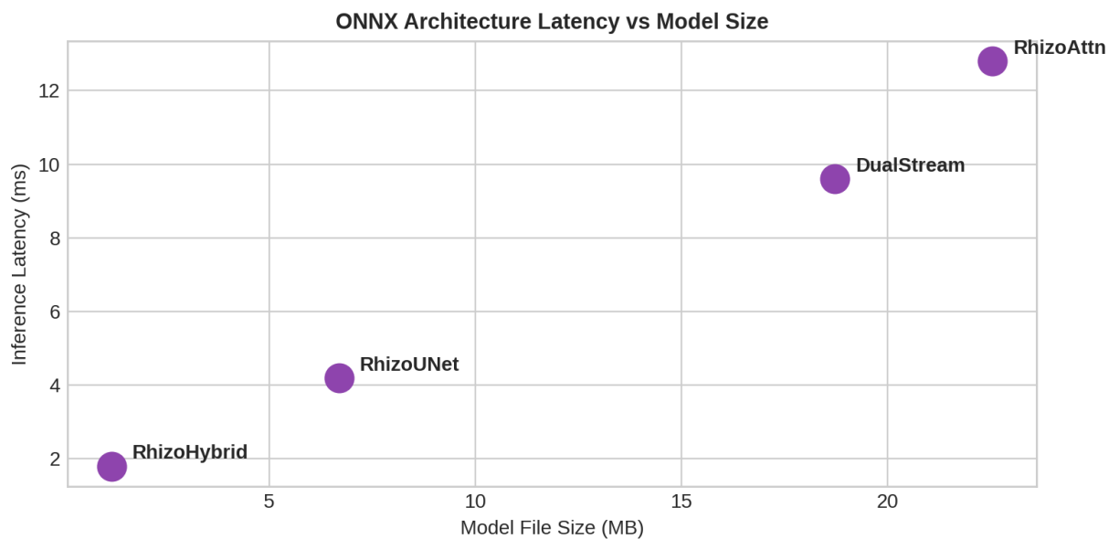
Figure 18: Figure 18: ONNX Model File Size vs Latency Profile
