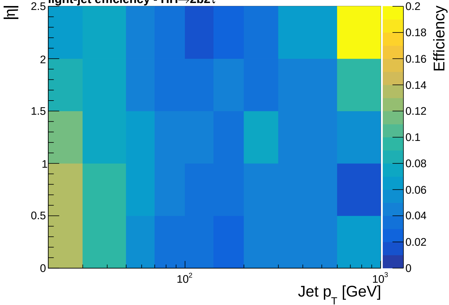
light-jet efficiency - HH \rightarrow 2b2\tau
