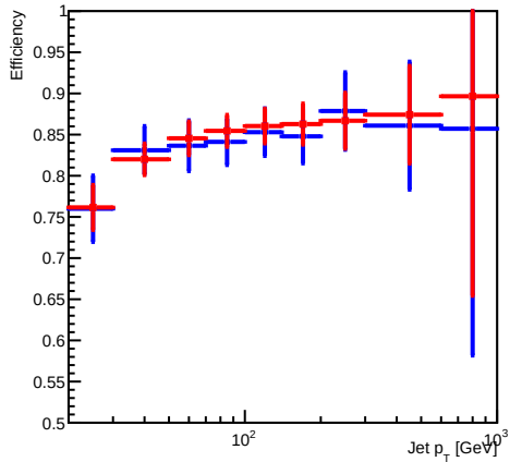
b-jet efficiency
