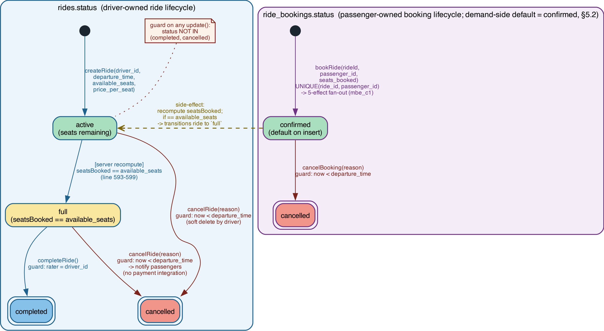
Ride + Booking state machines (carpooling.controller.js:511-709, migration 000)
