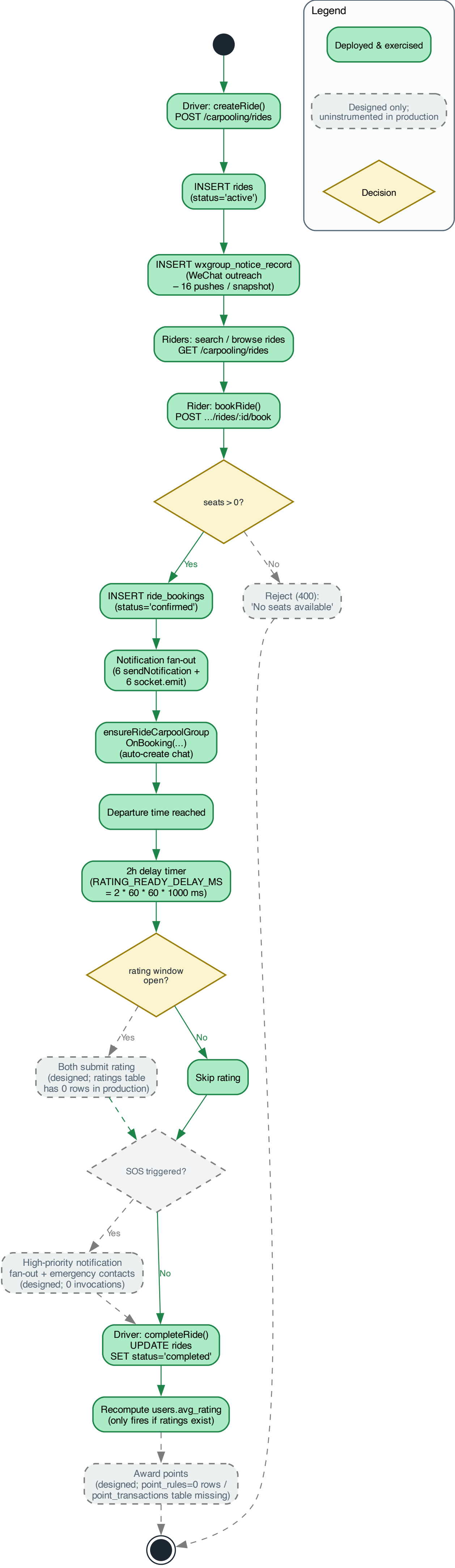
Full ride lifecycle activity diagram (createRide -> bookRide -> completeRide)
