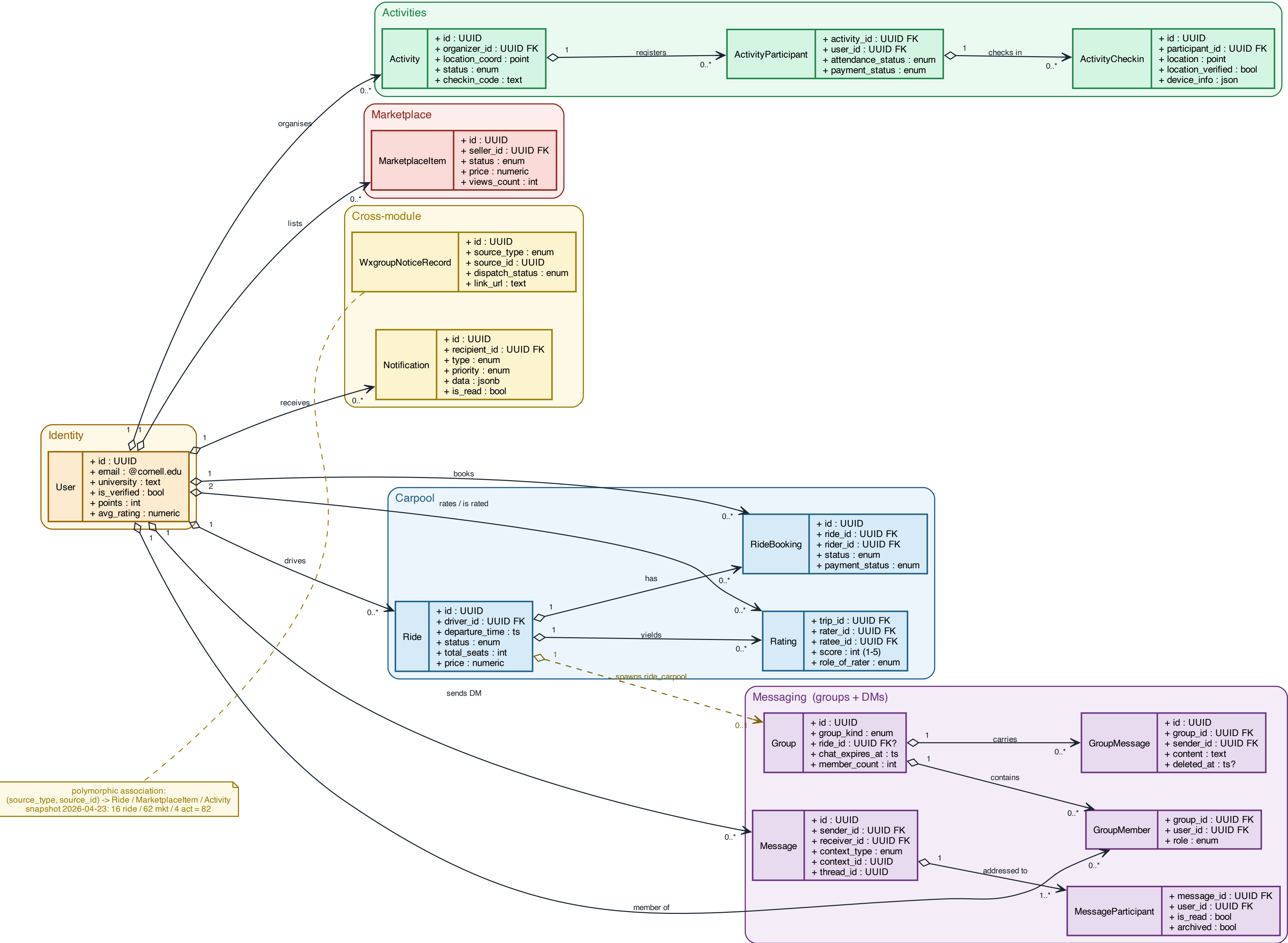
Class Diagram - production database schema (snapshot 2026-04-23) 15 core classes across 6 domain clusters; UML associations with multiplicity.
