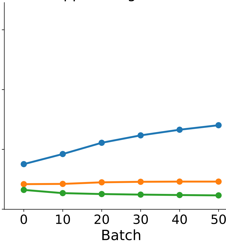
Approx.Degree = 3
