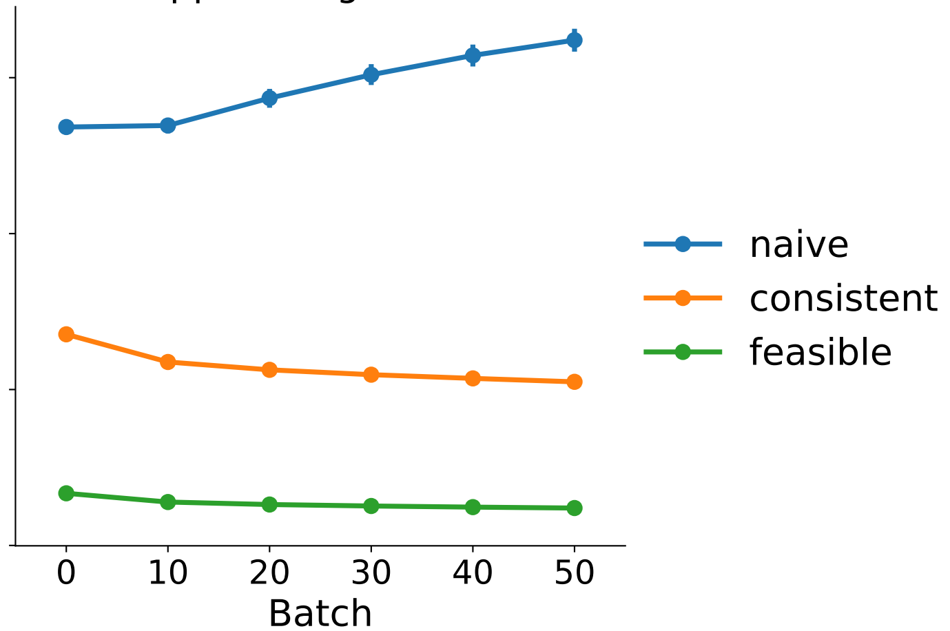
Approx.Degree = 4
