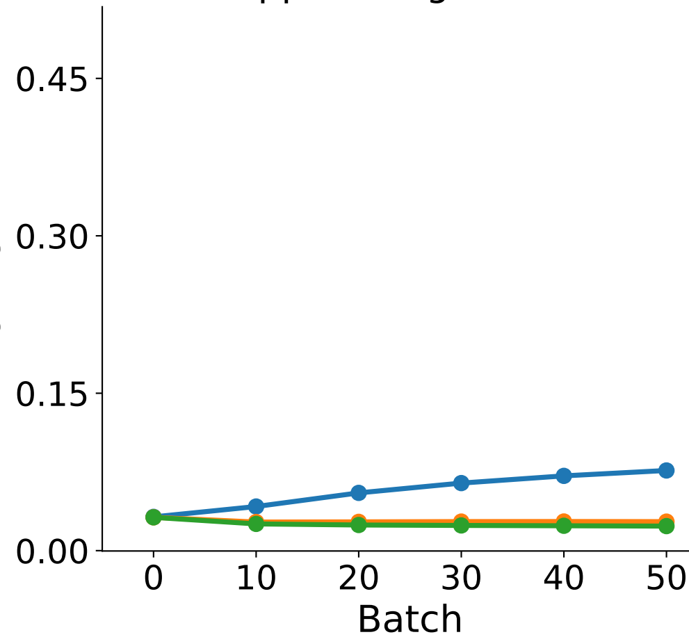
Approx.Degree = 1
