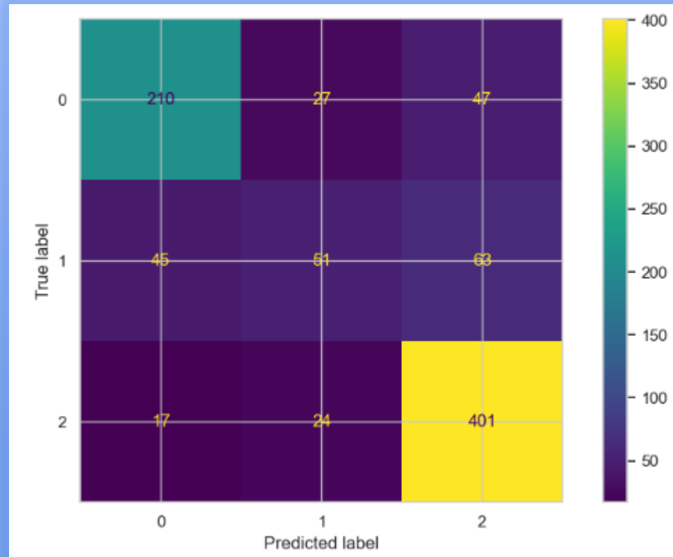
Confusion Matrix across 3 outcome classes (Graduate / Continue / Dropout)
