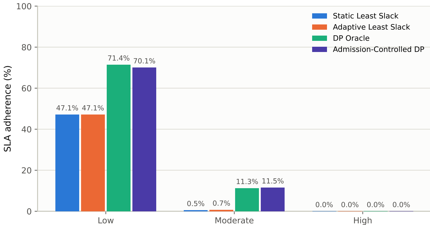
Offline simulation: SLA adherence by concurrency tier (1000-batch bootstrap, isolated per tier)
