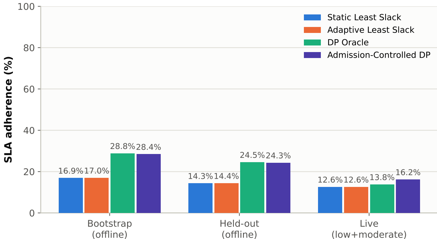
Aggregate scheduler ranking across evaluation methods
