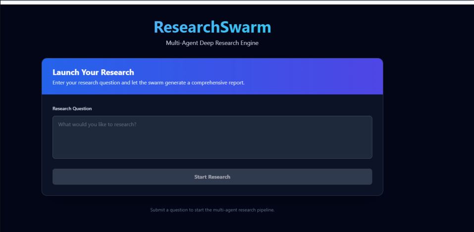
Launch Interface
