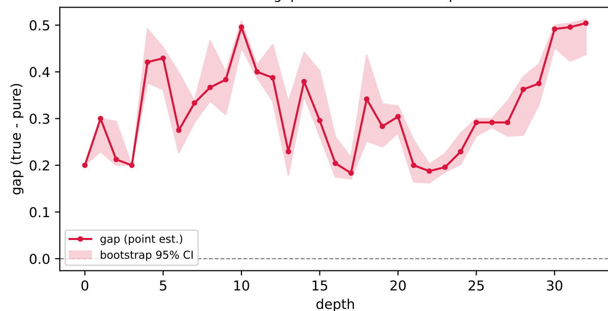
mistral-7b: sequence jackknife
