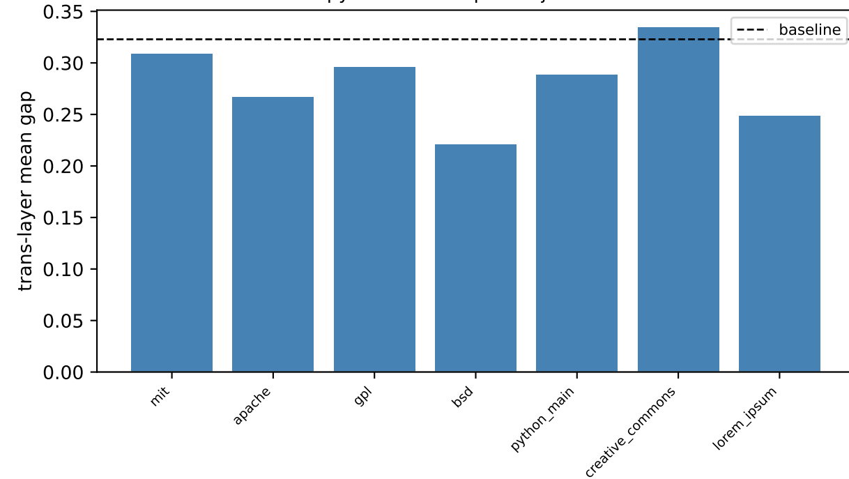
pythia-70m: sequence jackknife
