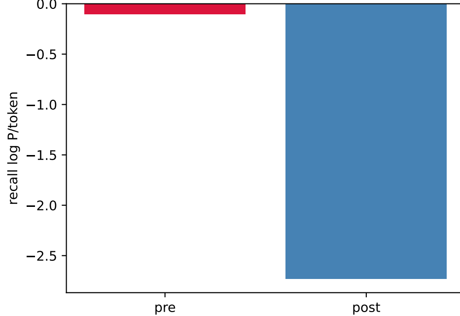
Memorized-pool recall
