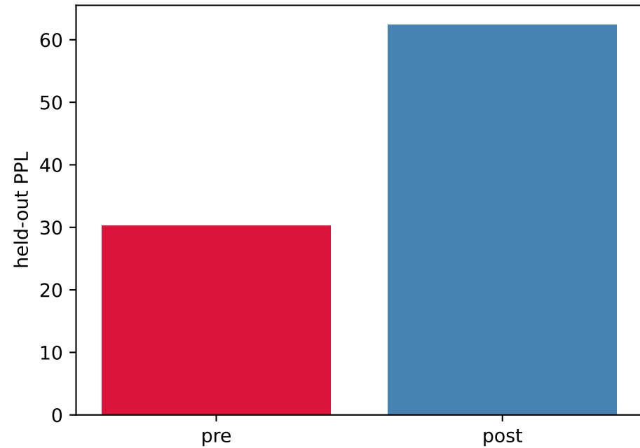
Capability (held-out)
