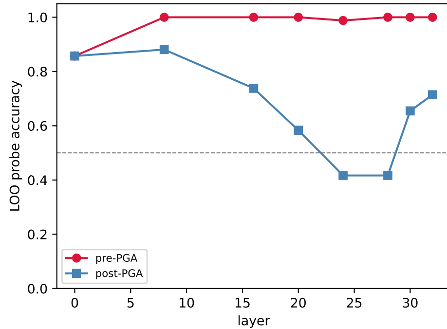
Probe collapse
