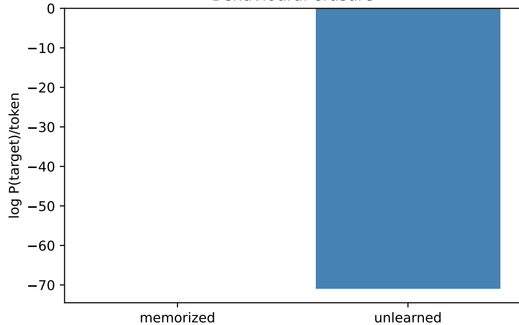
Behavioural erasure
