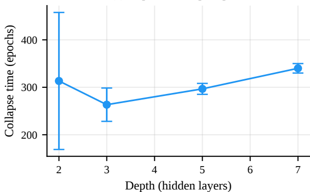
(a) Depth vs collapse speed
