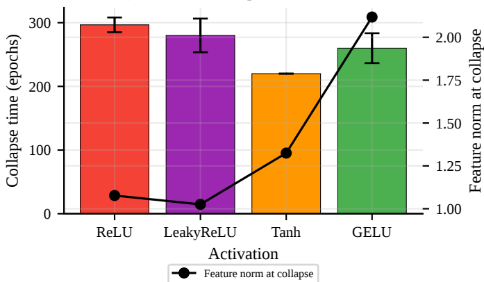
(b) Activation vs speed & threshold
