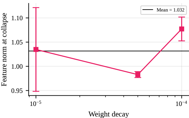
(c) Weight decay controls speed, not threshold CV = 0.059
