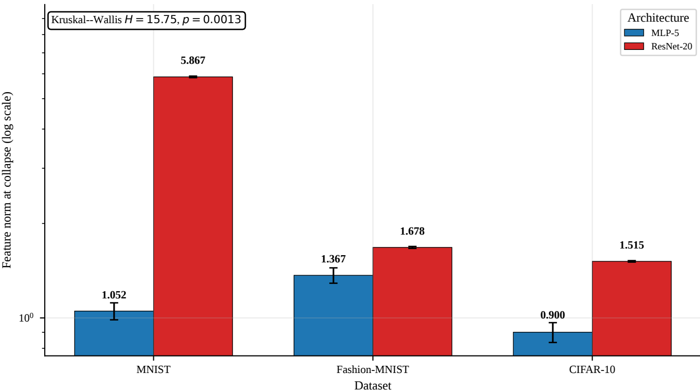
Feature norm at collapse by (model, dataset) pair
