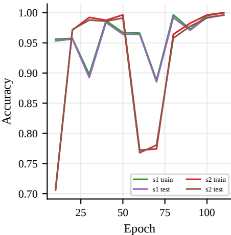
(a) Accuracy
