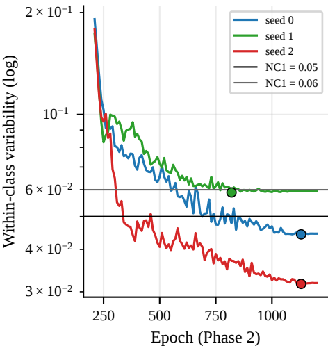
(a) SiLU NC1 plateaus
