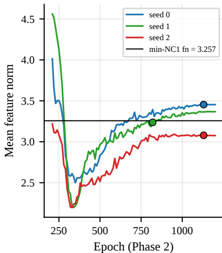
(b) Feature norm (dot=min NC1)
