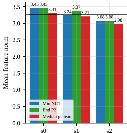
(c) Estimators agree ( \sim 5\% )
