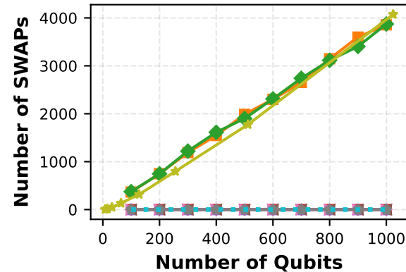
Linear Topology
