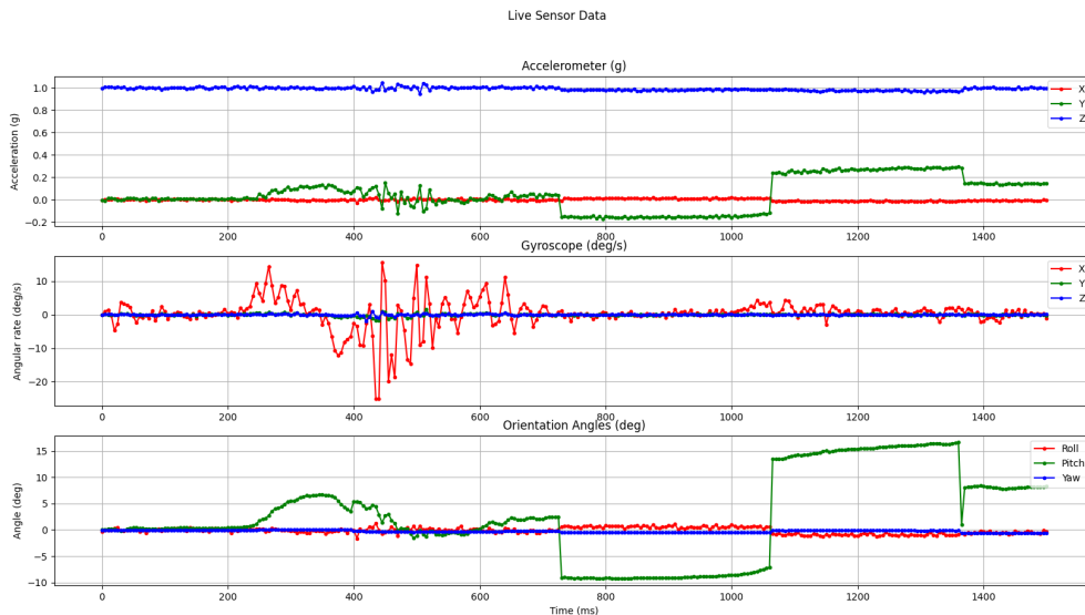
Figure 1: Gyro and Accelerator Sensor Data
