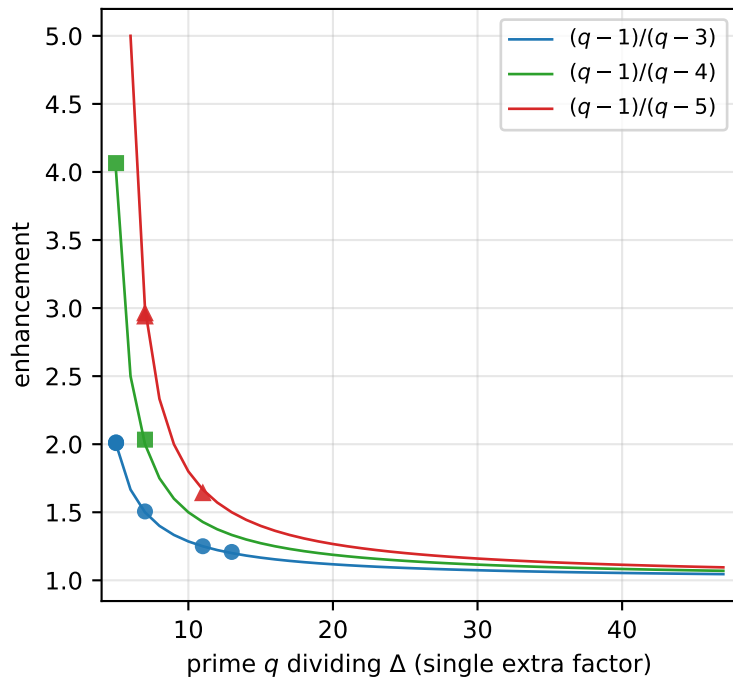
(B) per-prime gain (q-1)/(q-k)
