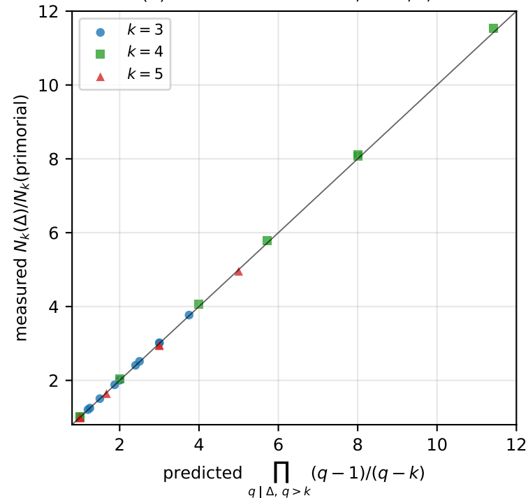
(A) unified resonance law, k = 3, 4, 5
