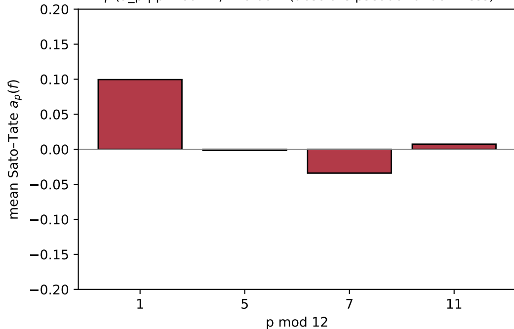
Test B — Langlands plume: a_p is congruence-immune \eta^2(a_p \mid p \bmod 12) = 0.002 (absolute pseudo-randomness)
