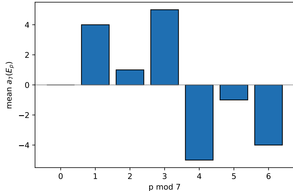
Test A — Galois fluid: a_7 IS a CRT coordinate \eta^2(a_7 \mid p \bmod 7) = 1.000 (absolute determinism)
